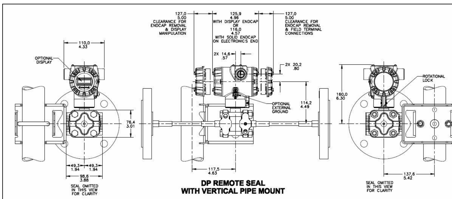
Reference Dimensions Vertical Mounting
