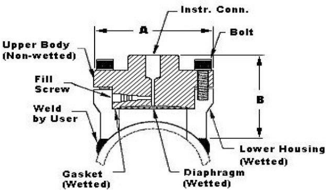
Figure 16— Seal Dimensions (3" Saddle Seal)
