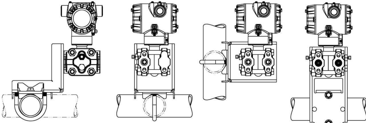
Figure 3 – Typical mounting configurations for STD810, STD815, STD820, STD830 and STD870 for reference
